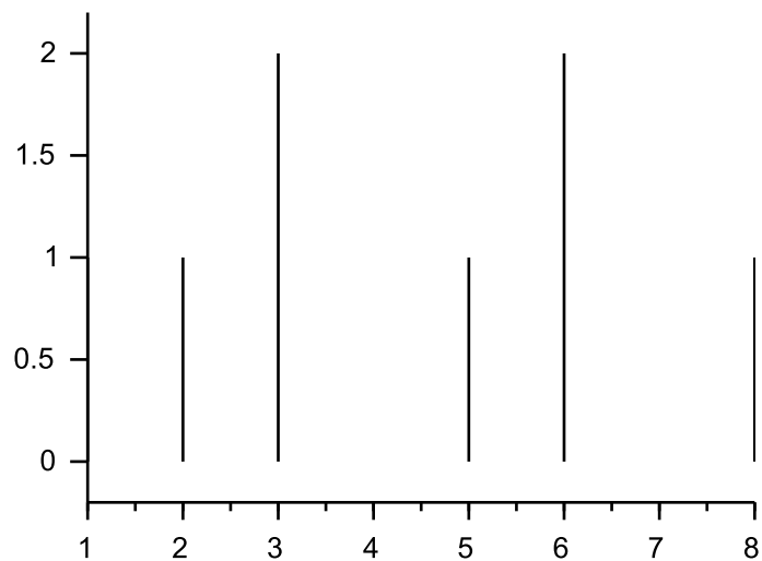
IDFT sequence
