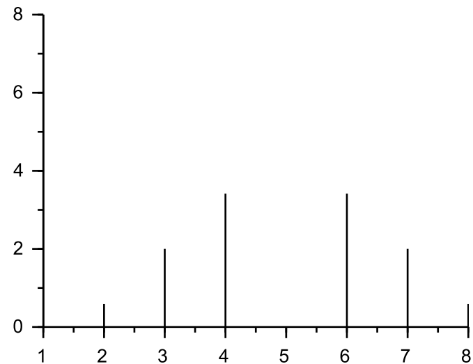
IDFT sequence
