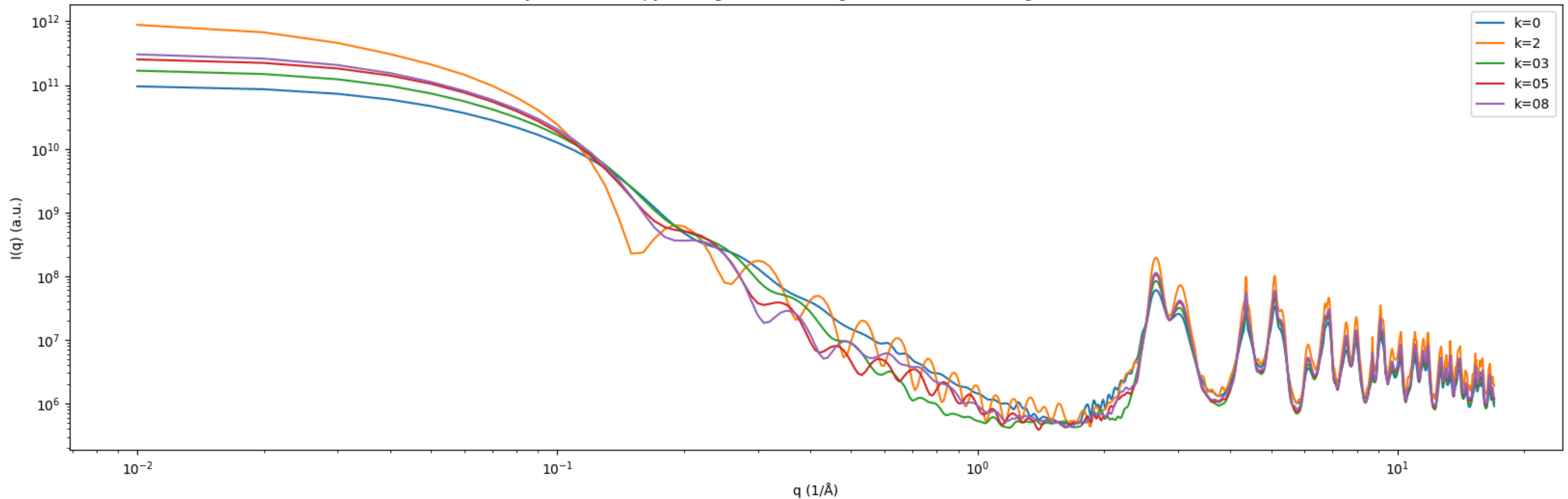
Debye curves of bipyramid growth (from a gold seed to core shell gold silver NP)
