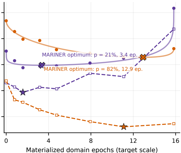
MARINER fit: simulated-epoching proxy
