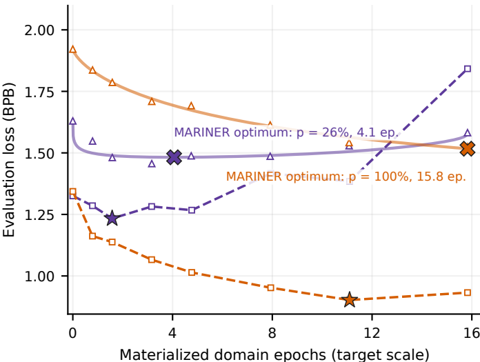
MARINER fit: proxy without simulated epoching
