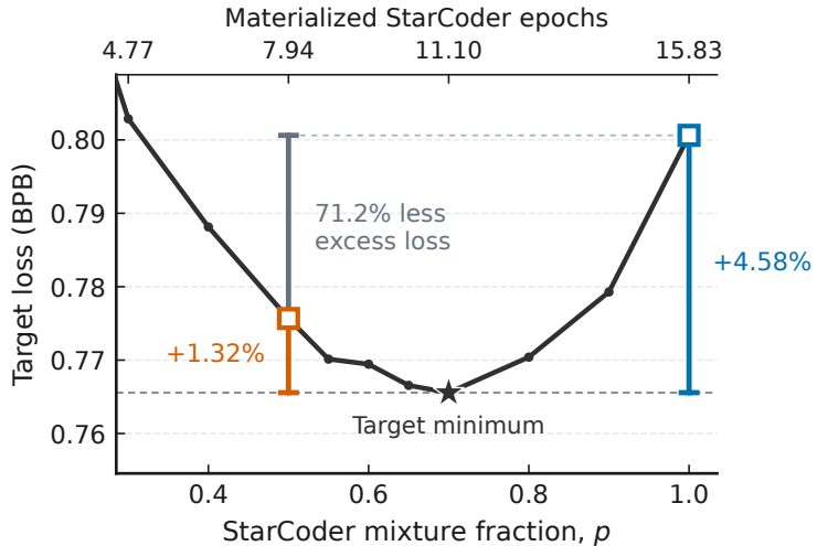
Target run ( 6.66 \times 10^{18} FLOPs)
