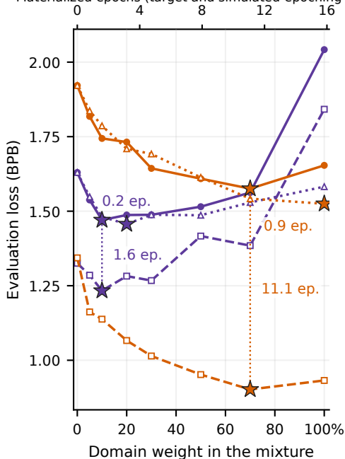
Proxy and target sweeps Dolmino FLAN: SciQ | FineMath-3+: GSM8K Materialized epochs (target and simulated-epoching proxy)
