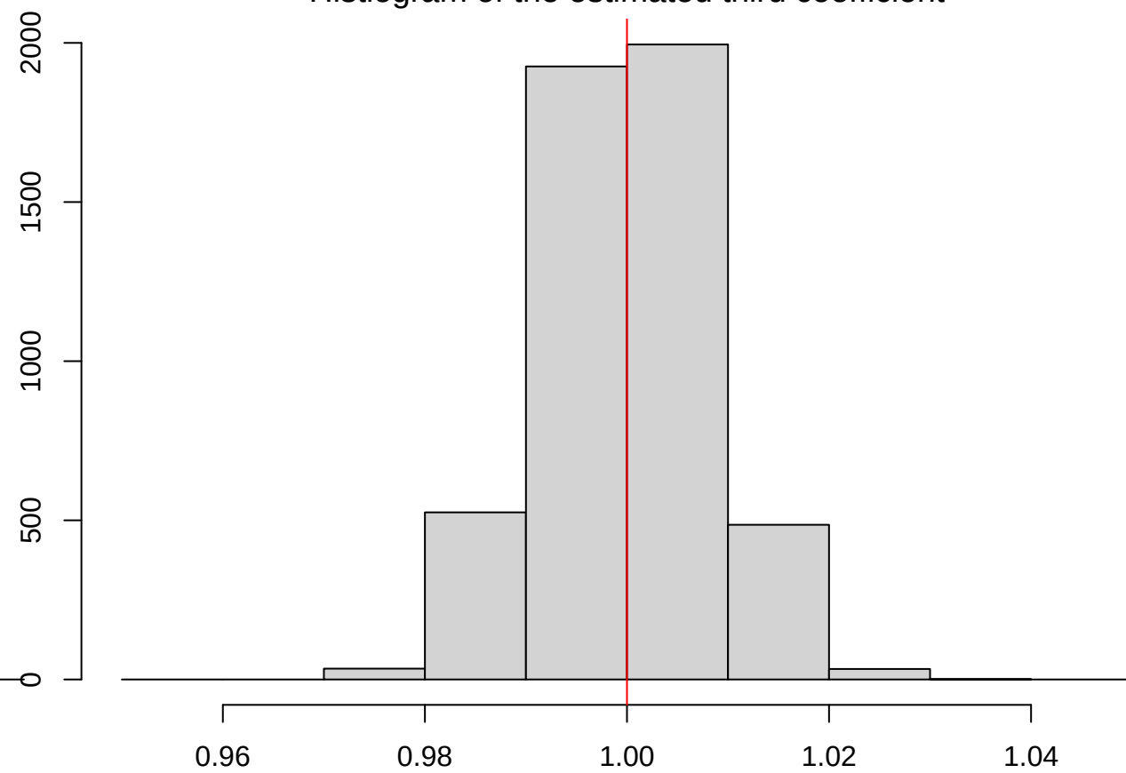
Histogram of the estimated third coefficient
