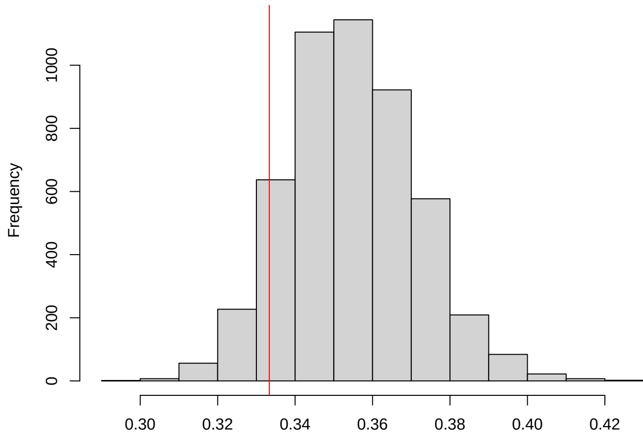
Histogram of the estimated square root of the long-run variance
