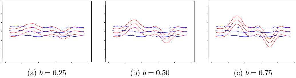
Figure 5: An example of two uniform confidence bands for T = 500 and b = 0.25, 0.50, 0.75 .
