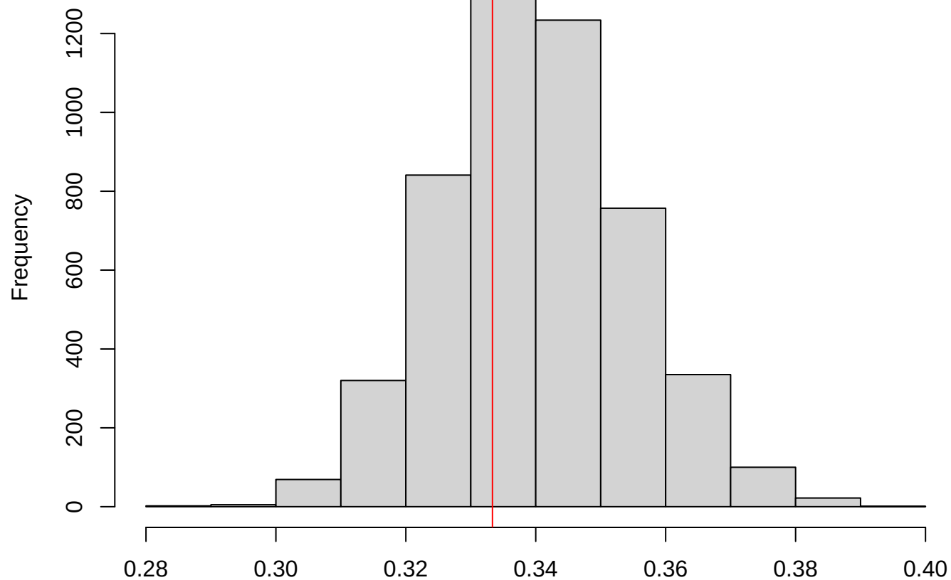
Histogram of the estimated square root of the long-run variance
