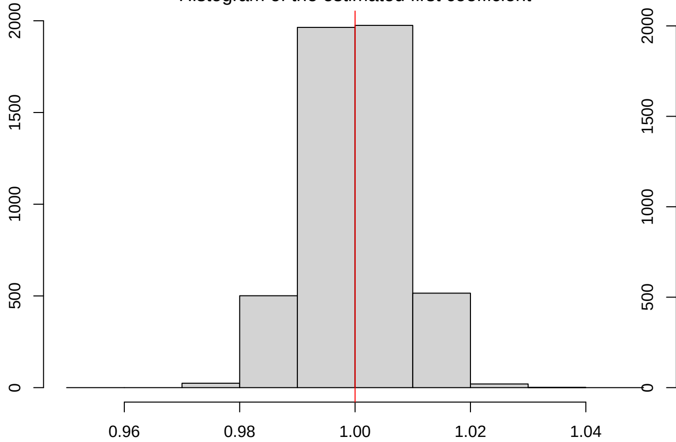
Histogram of the estimated first coefficient
