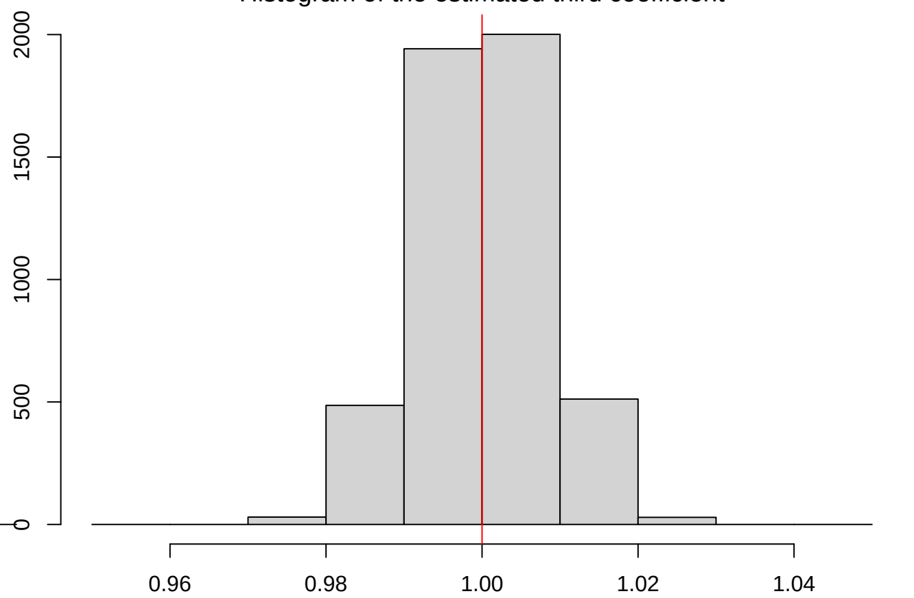
Histogram of the estimated third coefficient
