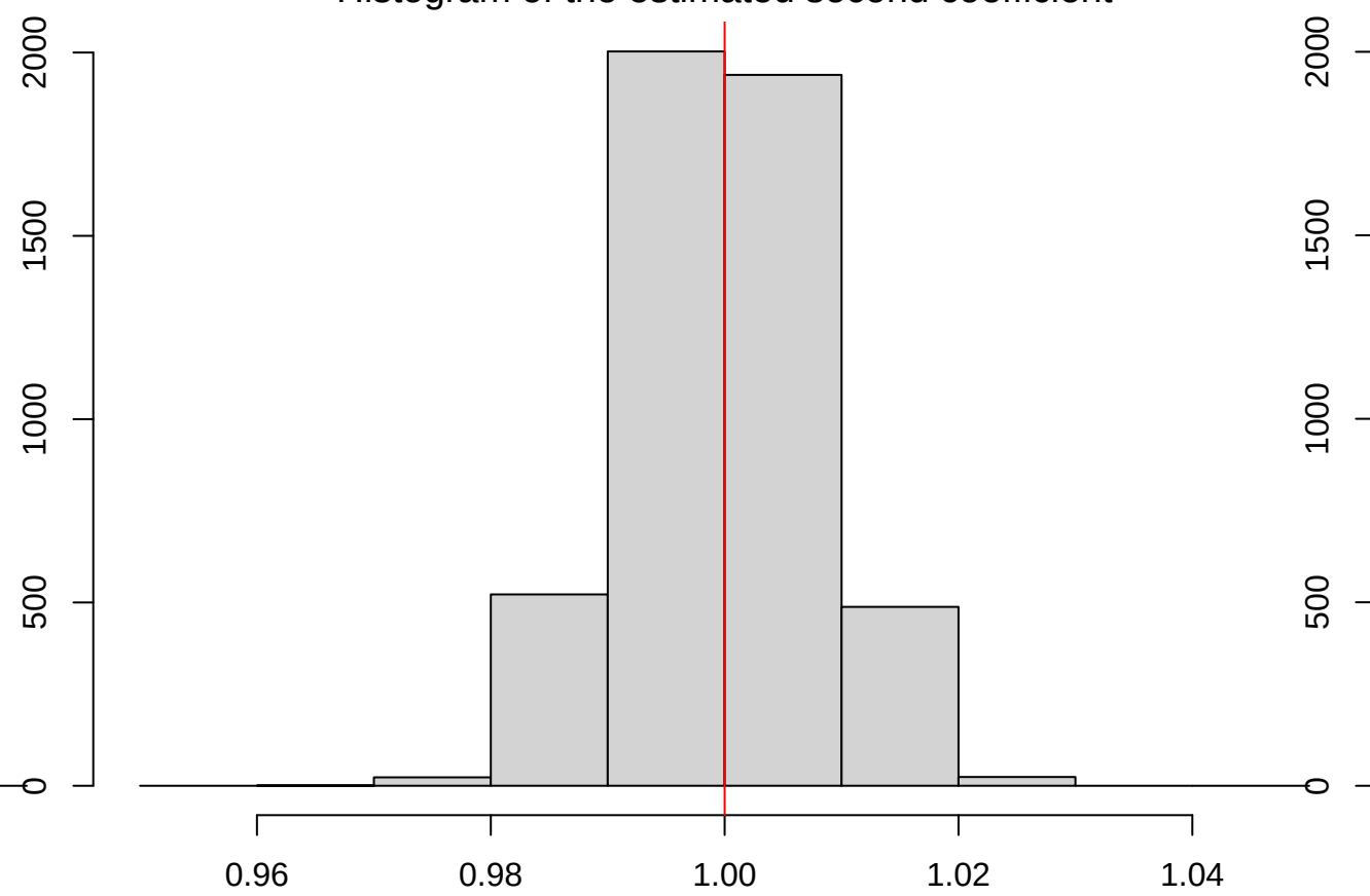
Histogram of the estimated second coefficient
