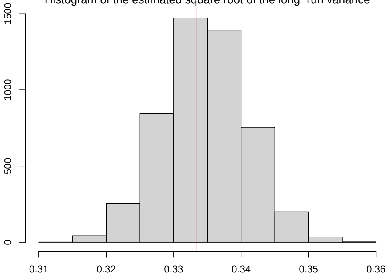
Histogram of the estimated square root of the long-run variance
