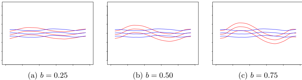
Figure 5: An example of two uniform confidence bands for T = 500 and b = 0.25, 0.50, 0.75 .
