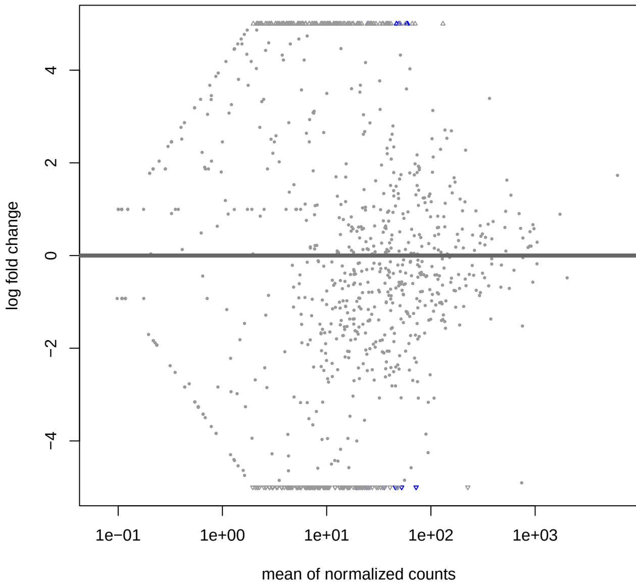
TnSeq MA Plot (Serum vs BHI)
