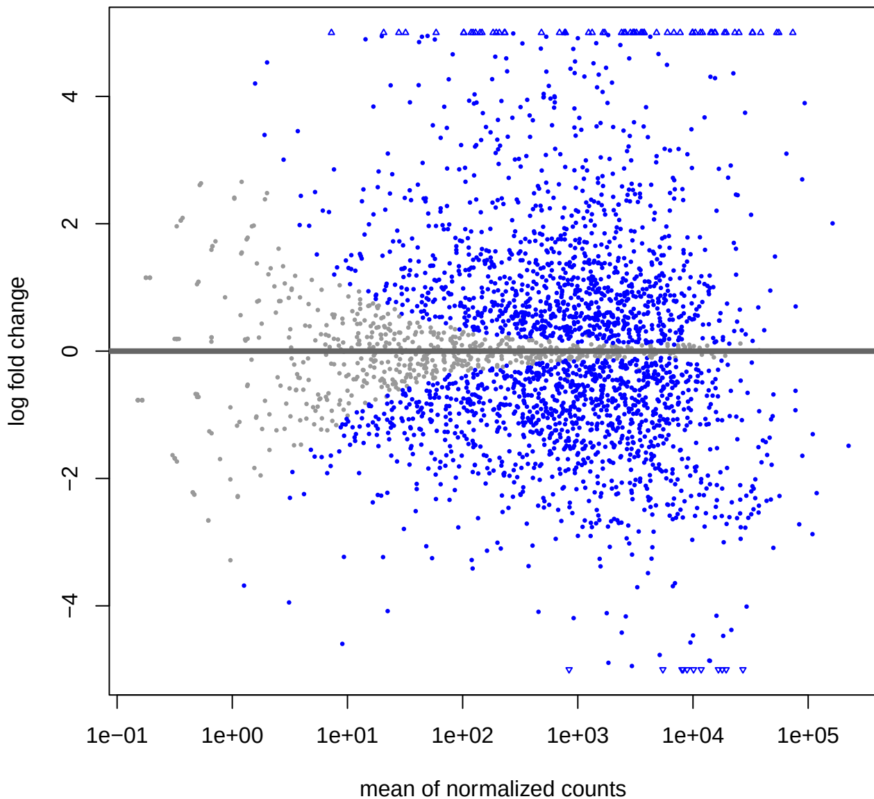
DESeq2 MA Plot (Serum vs BH)
