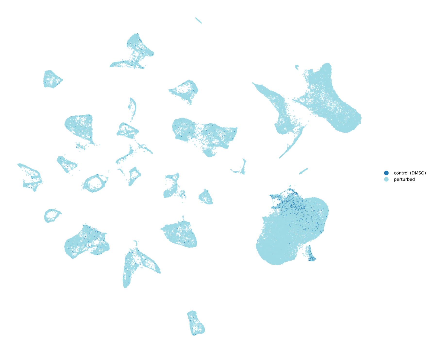
UMAP - coloured by treatment
