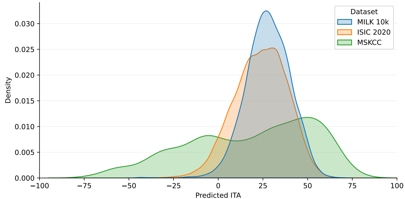
Predicted ITA distributions by dataset
