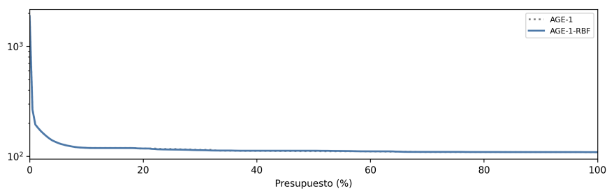
(c) f_{22}
