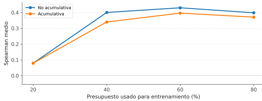
(c) SHADE
