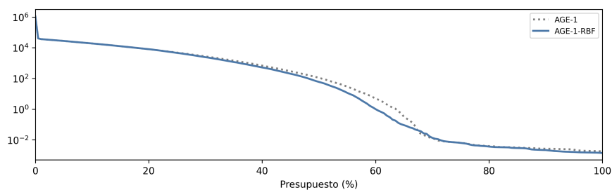
(a) f_3
