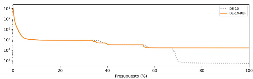
(c) f_{30}
