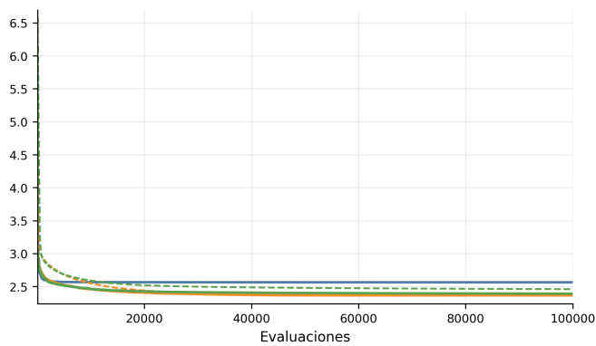
(c) f_{29}
