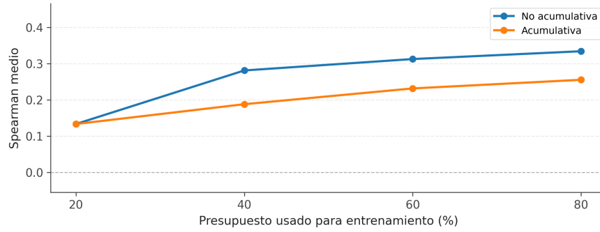
(a) AGE
