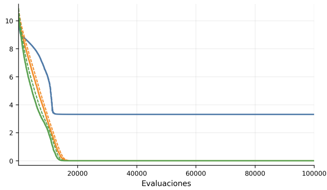
(a) f_1
