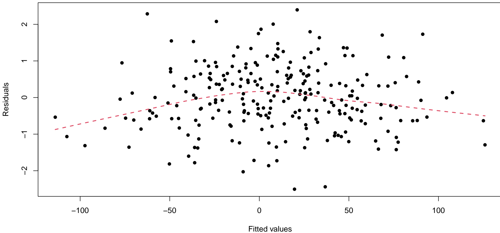
Residuals plot
