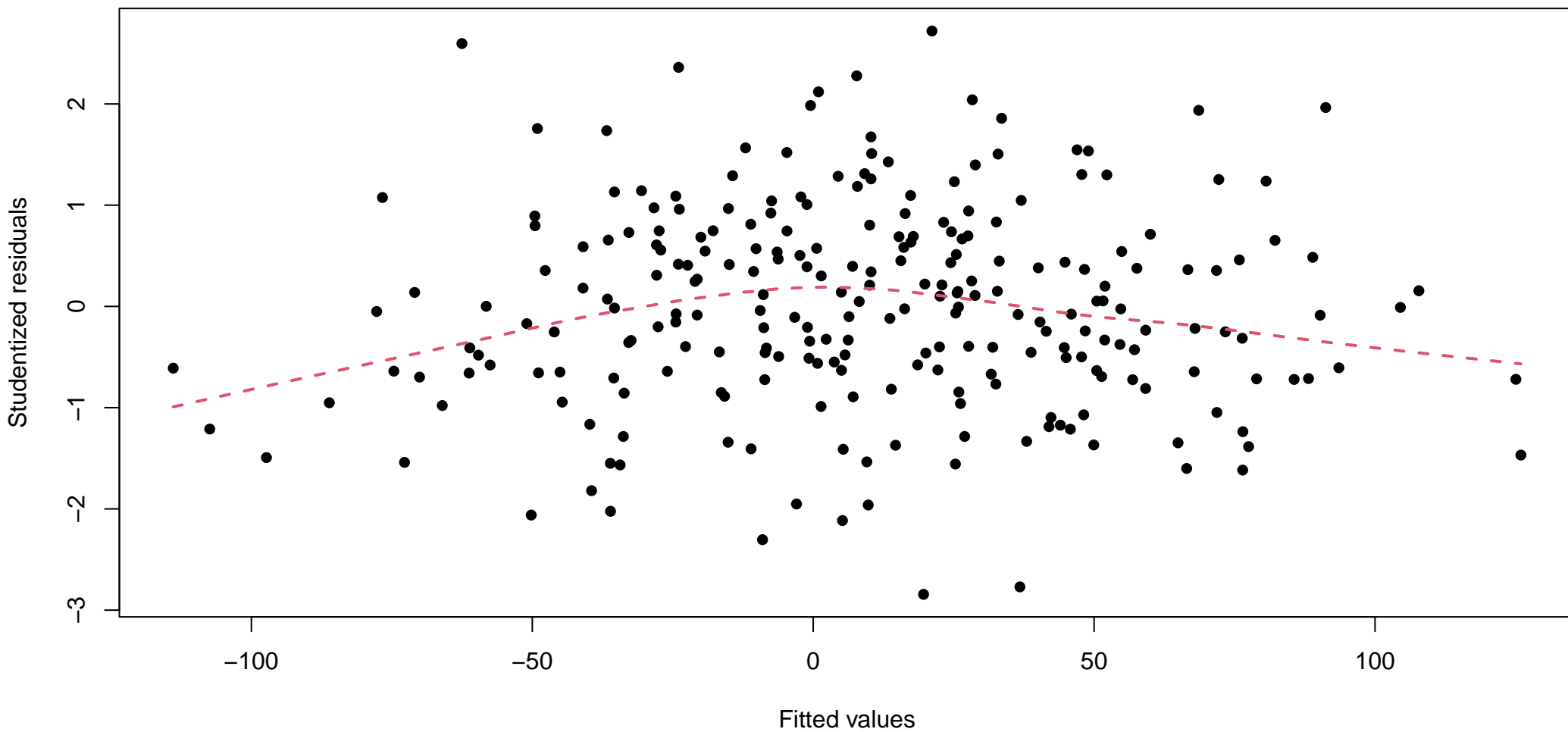
Studentized residuals plot
