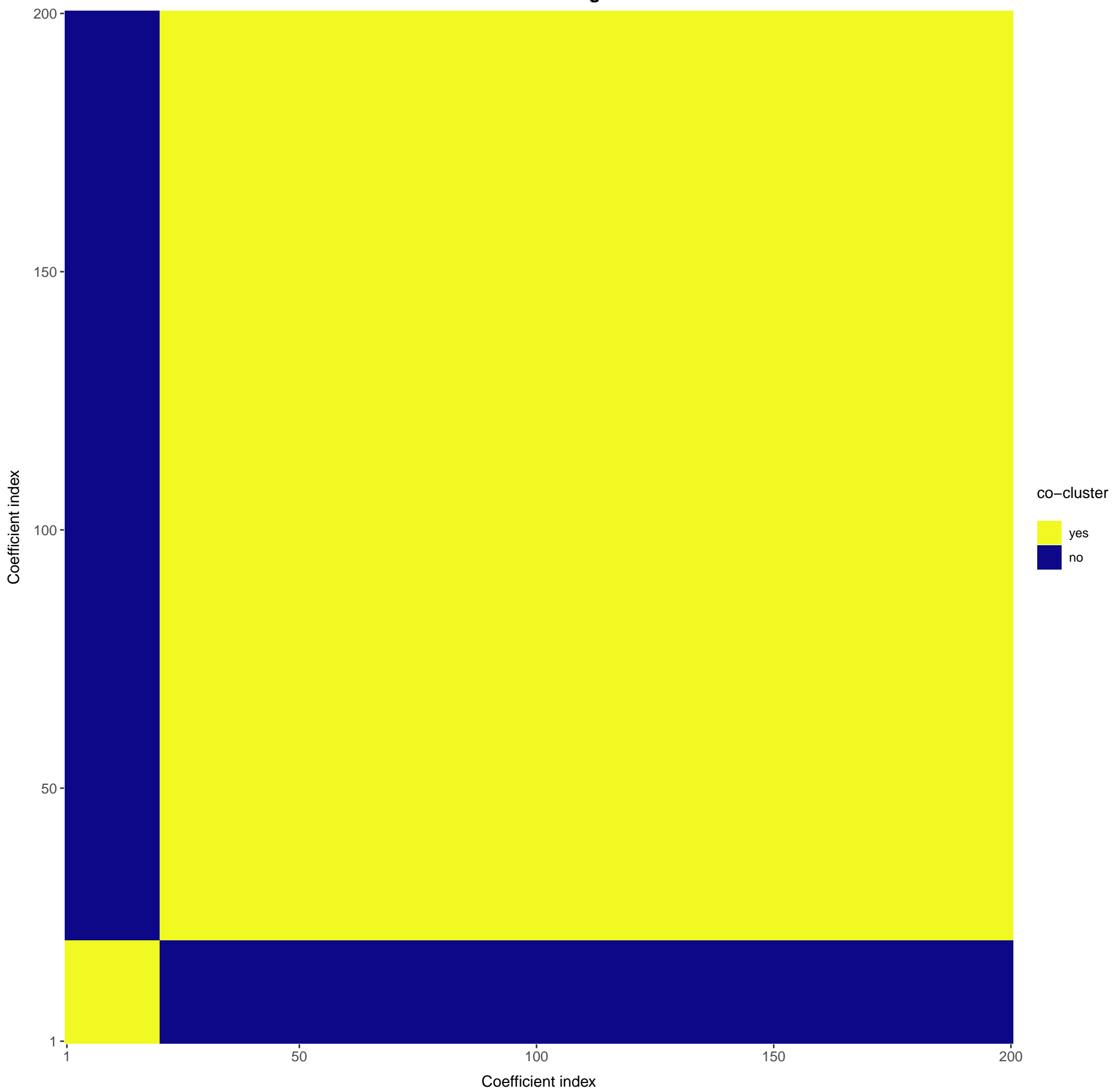
Co-clustering
