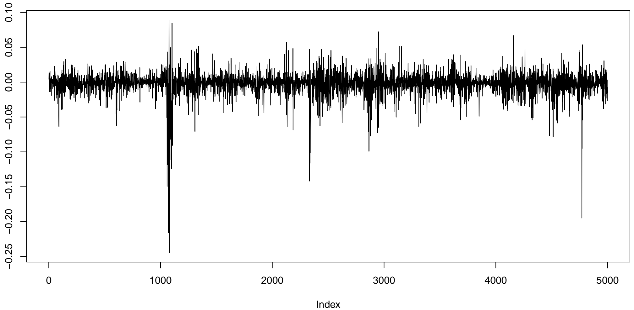
beta_200
