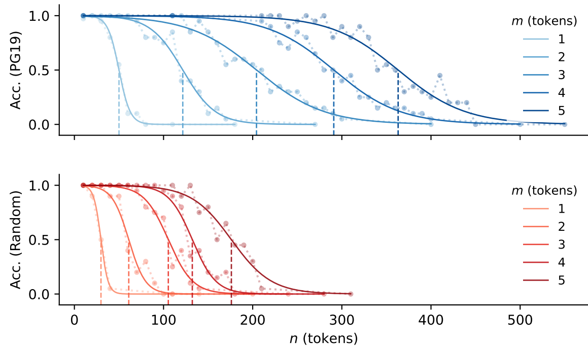
Qwen2.5-1.5b
