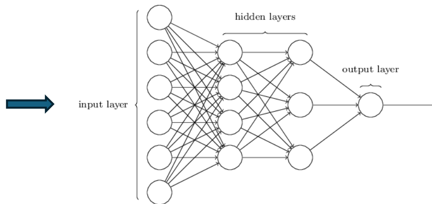
Reti neurali, 1986
