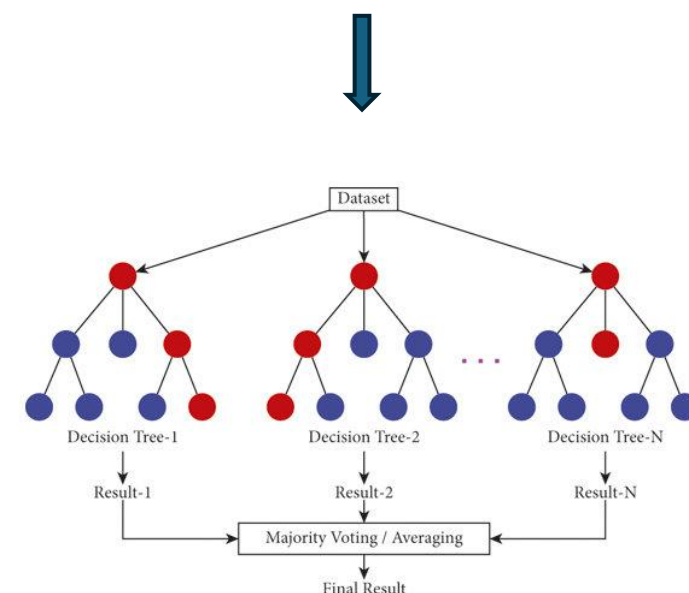
Random Forest, 2001
