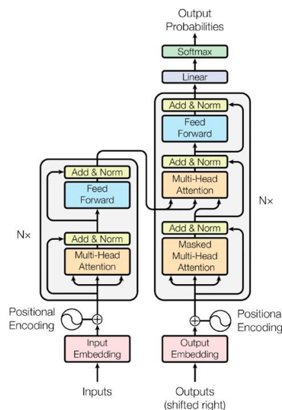
Transformers, 2017
