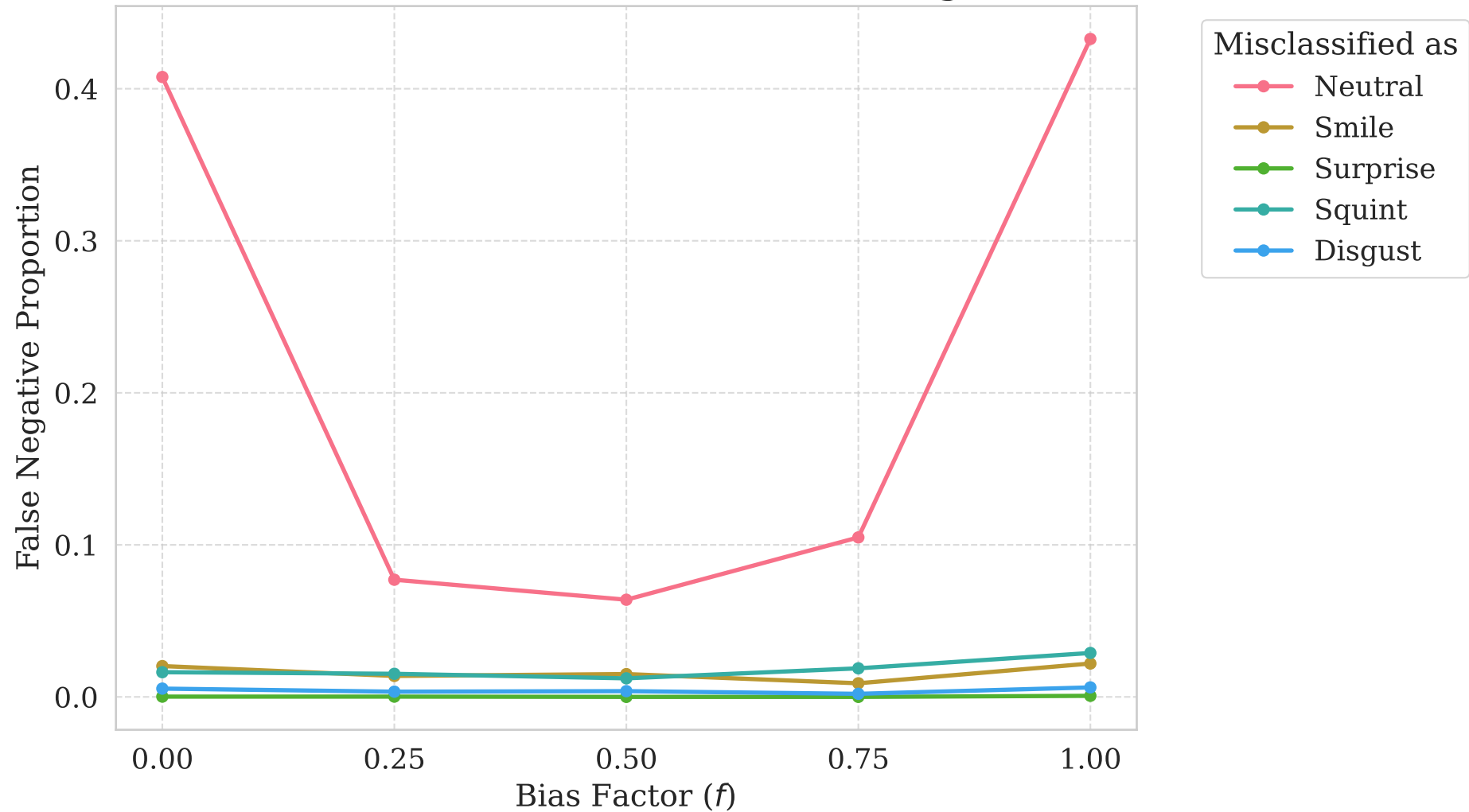
Error Distribution under Bias Variation - Target: Scream
