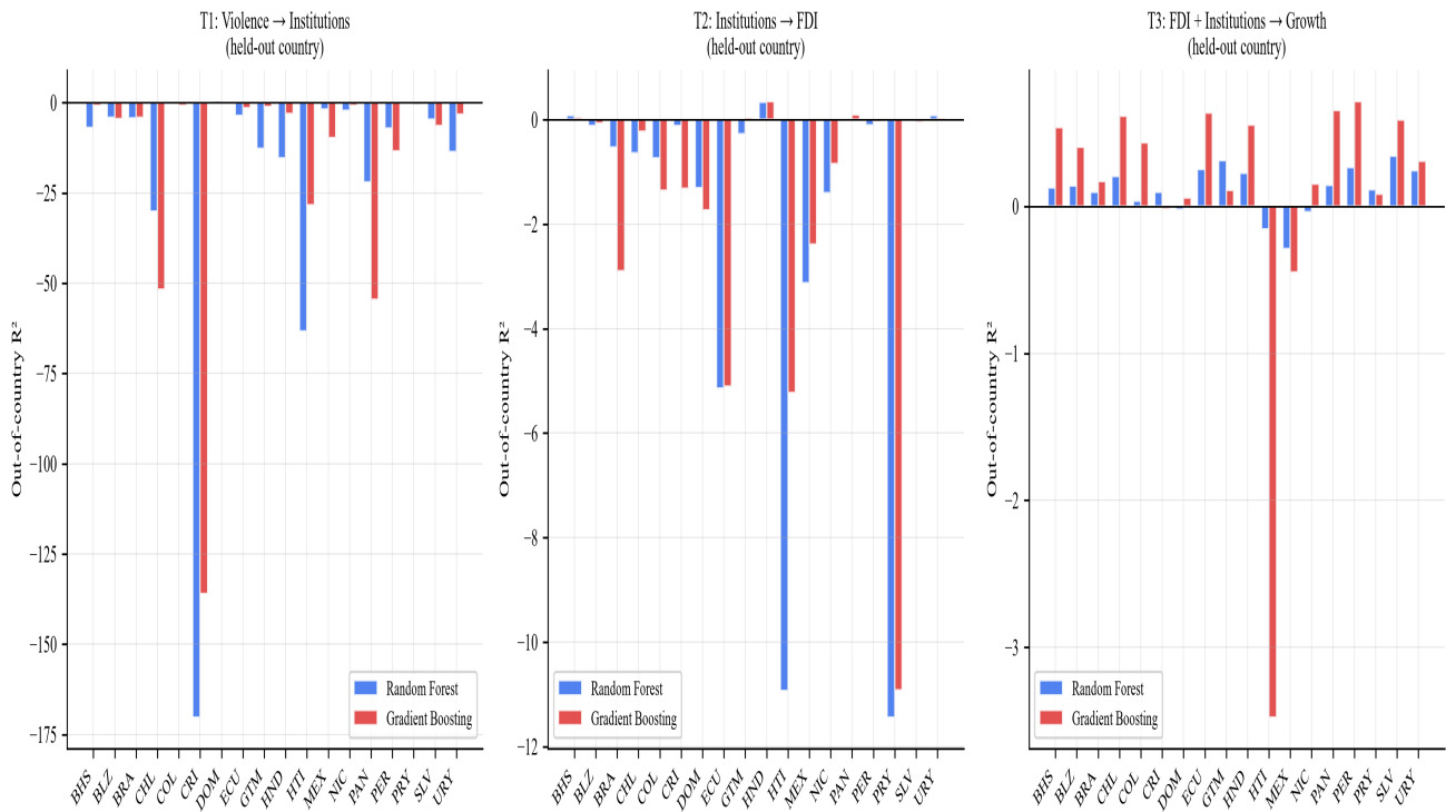
Figura 8 — LOCO-CV R^2 por país Leave-One-Country-Out Cross-Validation (LOCO-CV) Random Forest & Gradient Boosting | Note: G=18 folds → wide uncertainty
