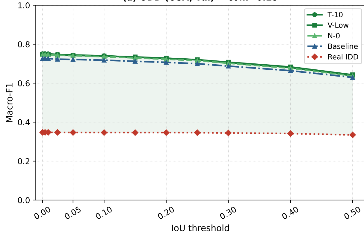
(a) ODD (USA, val) -- conf=0.25
