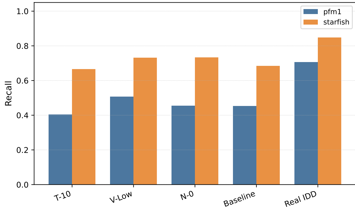
IDD (ITA, test) -- recall by class (conf=0.25, IoU=0.001)
