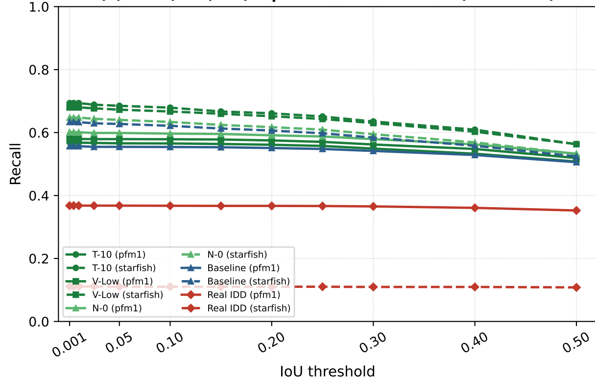
(a) ODD (USA, val) -- per-class recall vs. IoU (conf=0.25)
