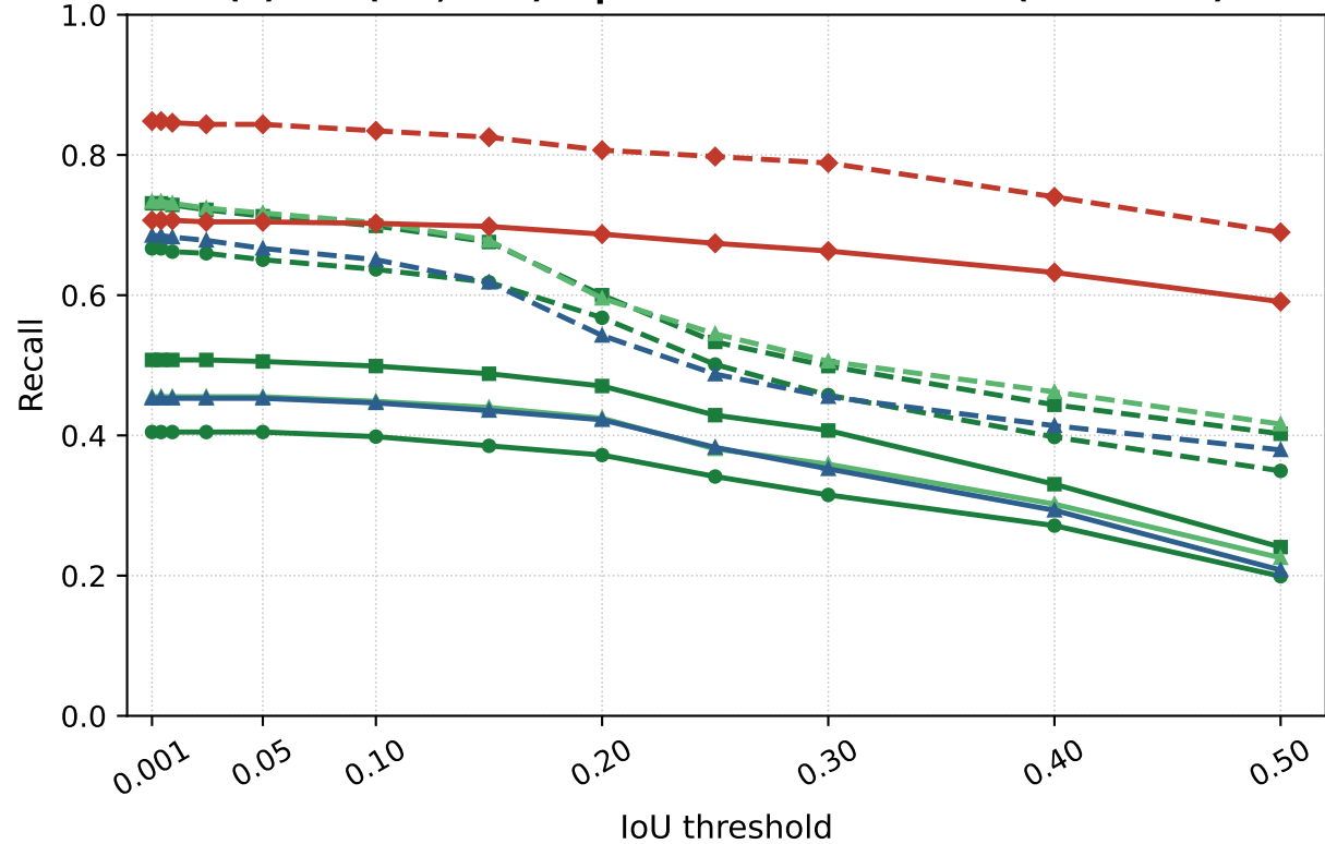
(b) IDD (ITA, test) -- per-class recall vs. IoU (conf=0.25)
