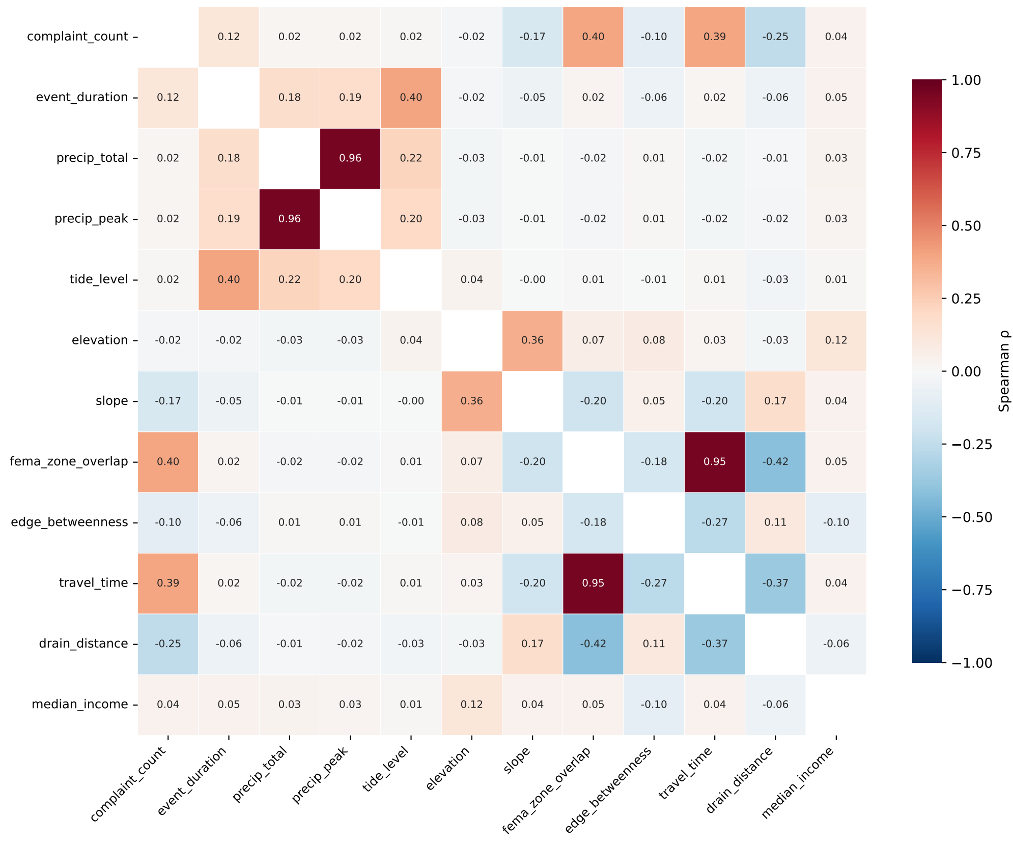
Spearman Correlation Matrix — BN Variables
