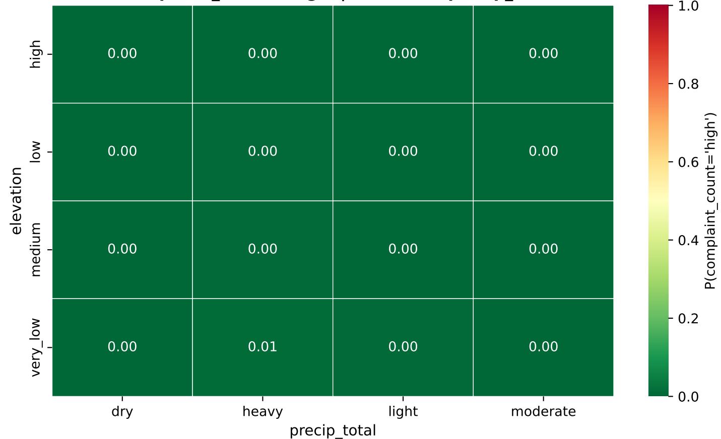
P(complaint_count='high' | elevation, precip_total)
