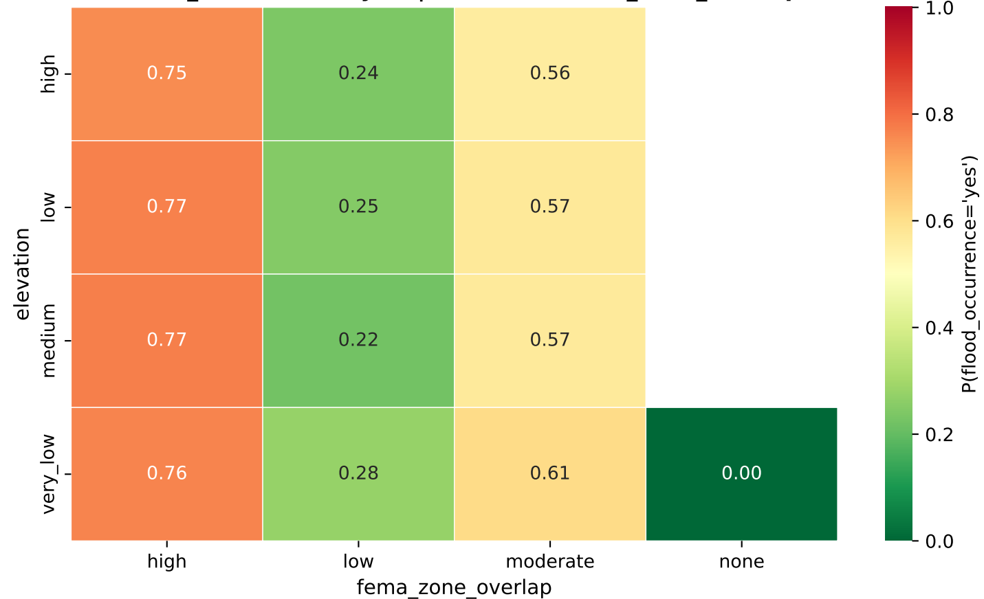
P(flood_occurrence='yes' | elevation, fema_zone_overlap)
