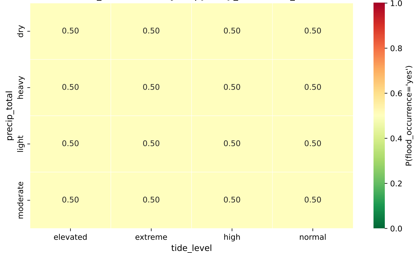
P(flood_occurrence='yes' | precip_total, tide_level)
