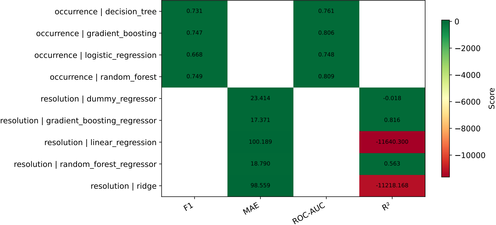
Model Performance Summary — All Tasks (Temporal Split)
