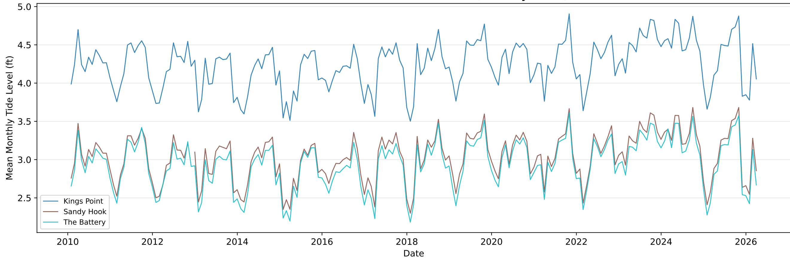
Tidal Observations — NOAA Stations (Monthly Mean)
