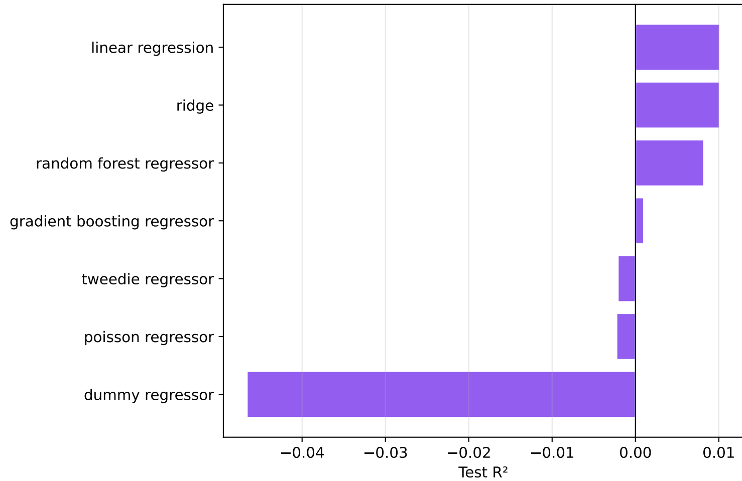
Intensity Regression R^2 by Model (Temporal Split)
