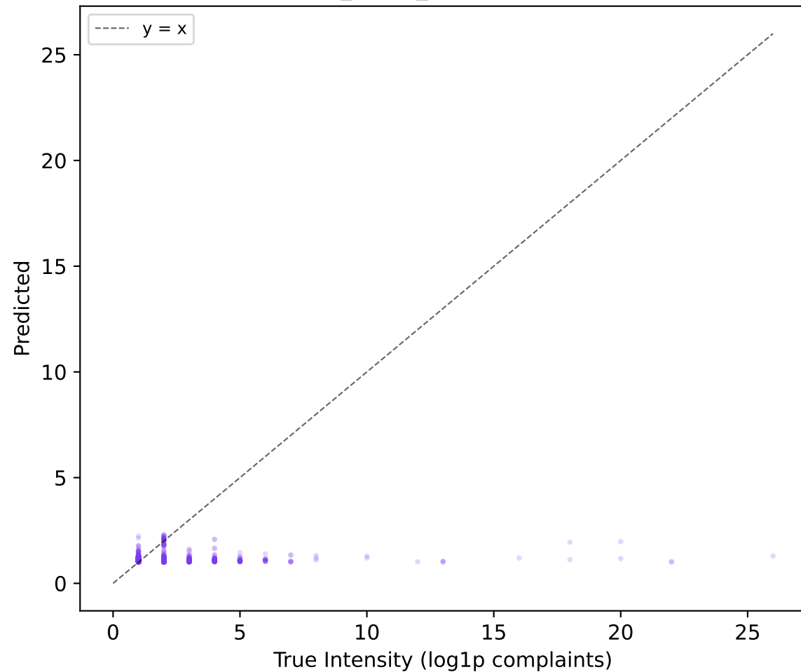
Intensity: Predicted vs. Actual (random_forest_regressor, test set)
