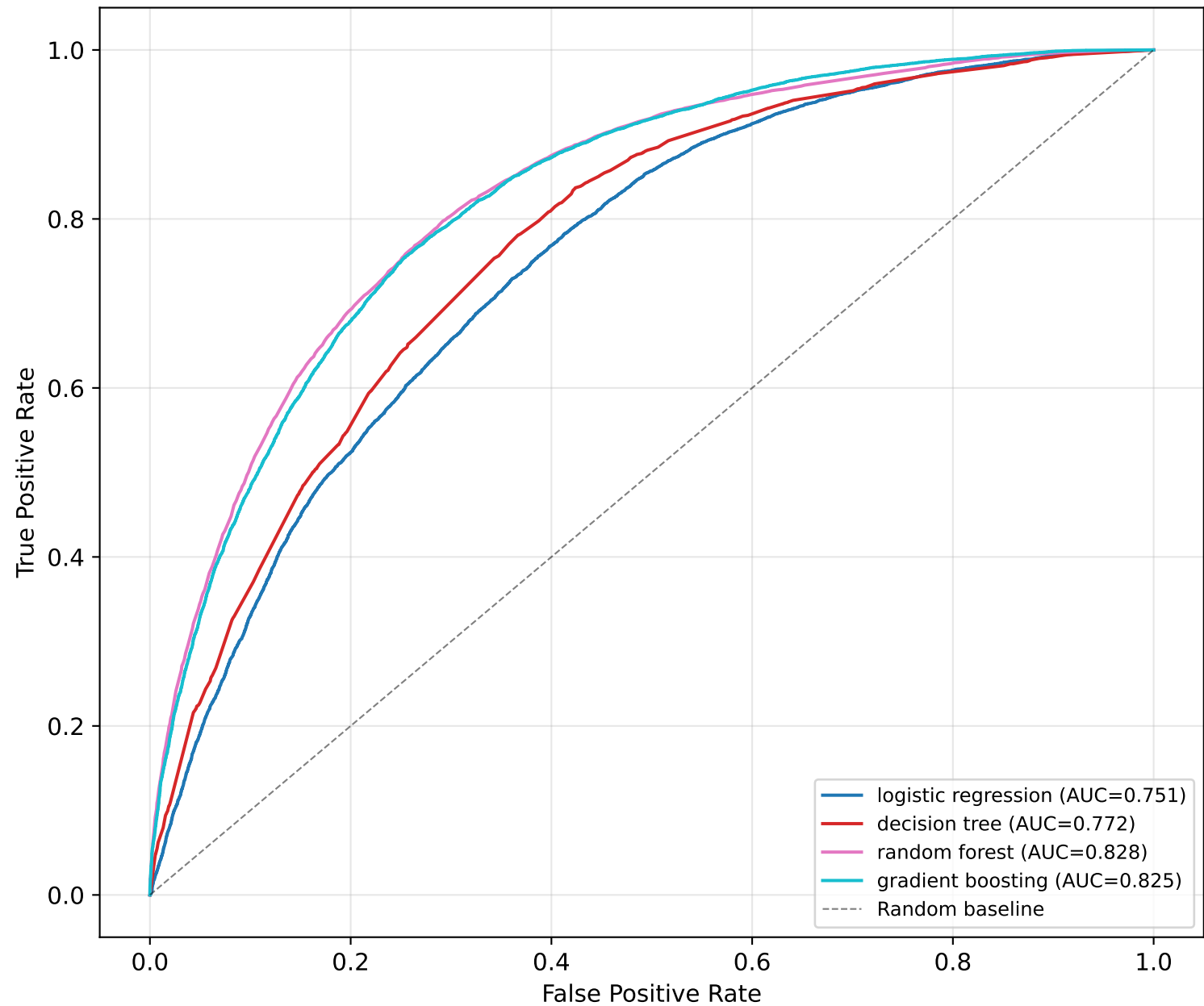
ROC Curves — Flood Occurrence Classification (Test Set)
