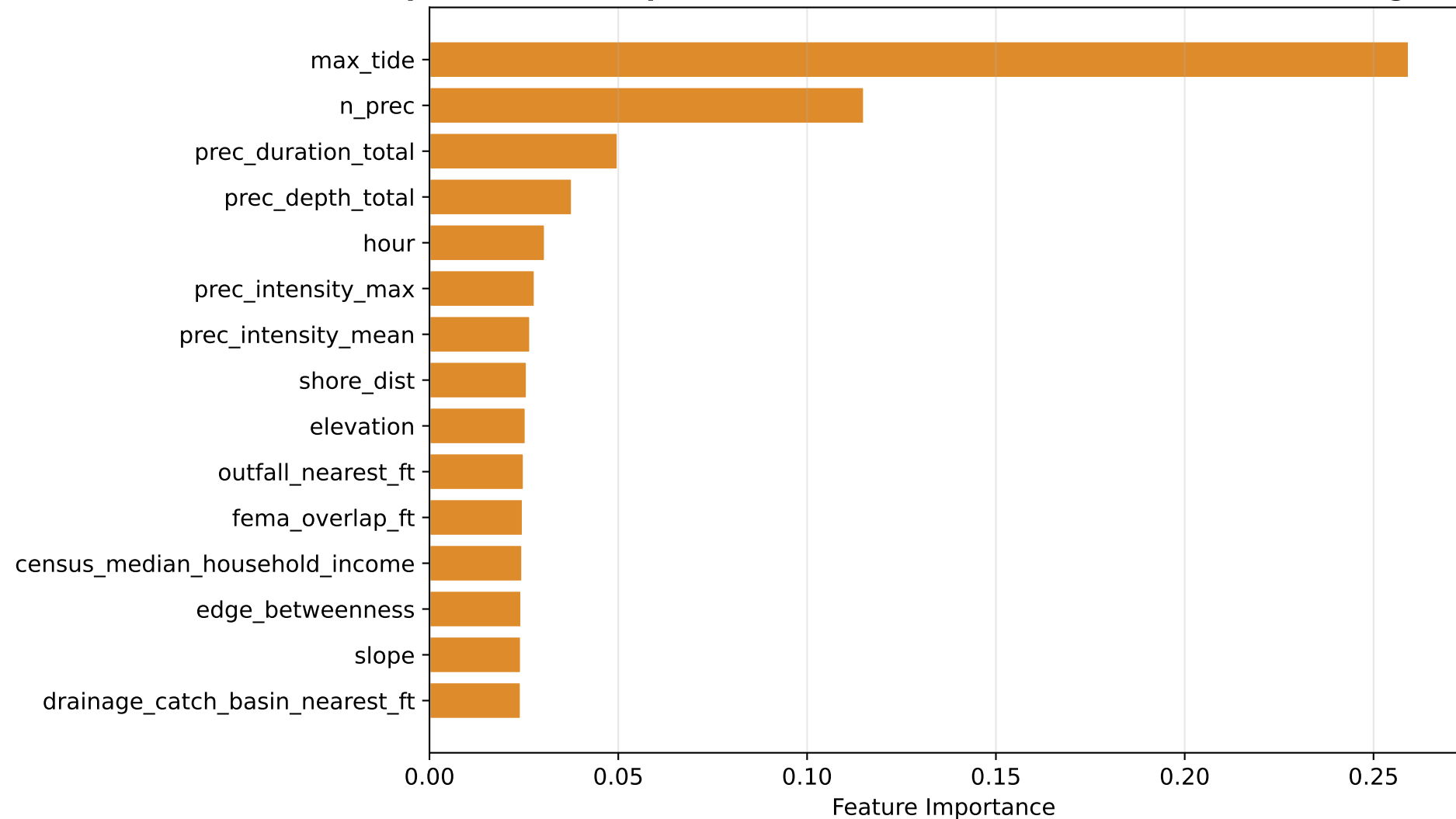
Top 15 Feature Importances — Resolution Time (Random Forest Regressor)
