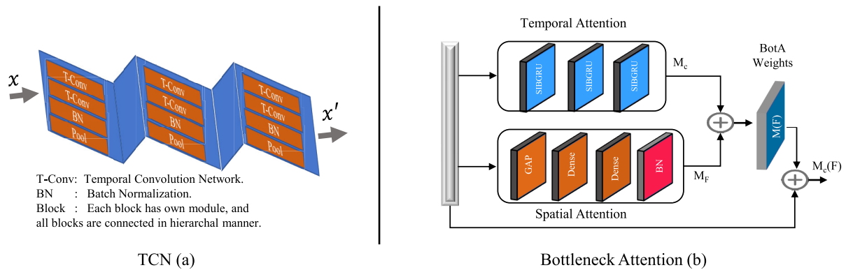
FIGURE 2. Overview of the proposed ST-TCN (a) and bottleneck attention (b) modules. All blocks are hierarchically interconnected in TCN and parallel in Bottleneck attention.
