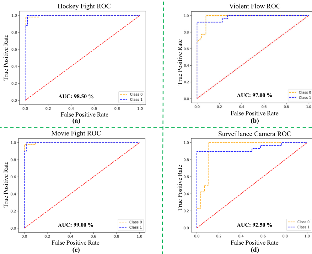
FIGURE 6. The proposed violence detector ROC curves.
