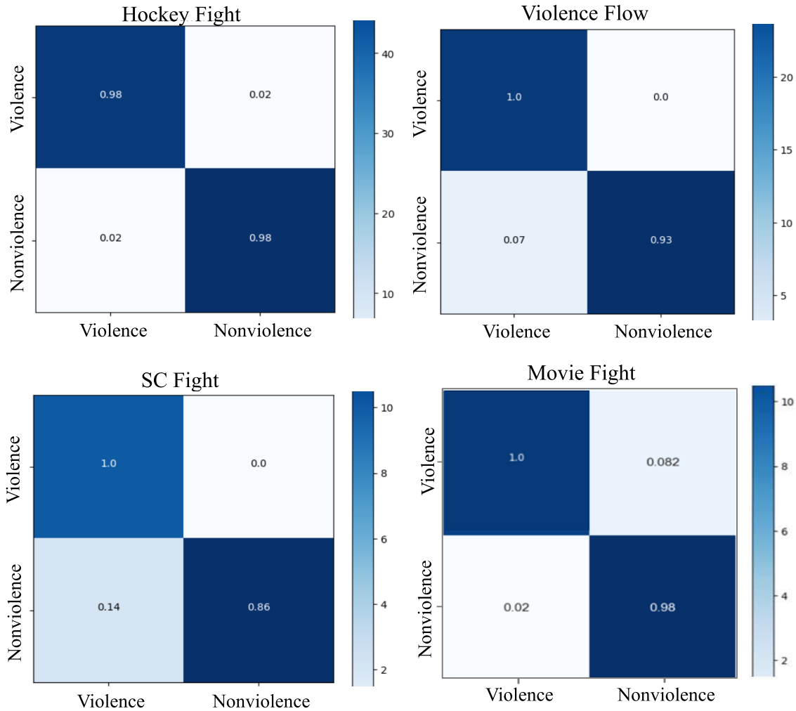
FIGURE 5. The confusion among each dataset's actual and predicted values to better understand the model's performance.
