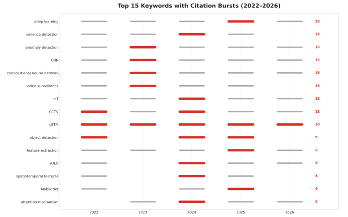
Fig. 5. Top 15 keywords with the strongest citation bursts — red segments indicate heightened activity.
