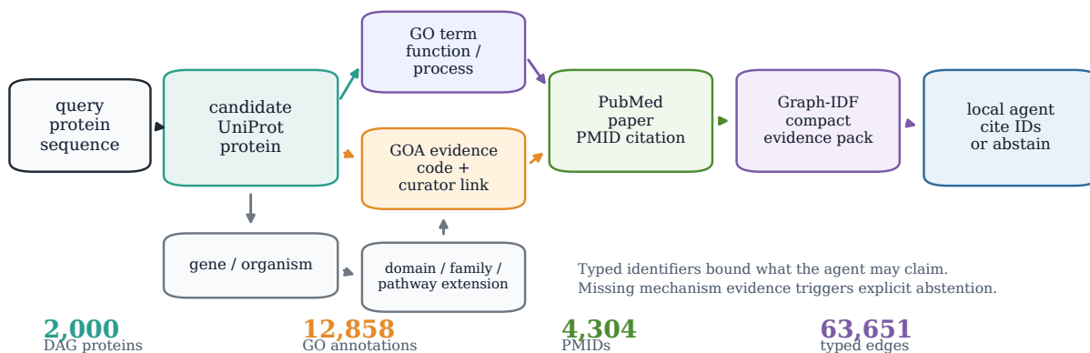
Figure 3: BioRAG-SeqLit-DAG application path. A held-out protein sequence retrieves candidate proteins, traverses curated GO/GOA-to-PubMed relations, and is compressed by a Graph-IDF selector into a citation-bounded Agent evidence pack. Typed identifiers limit valid claims, while absent mechanism evidence triggers abstention.
