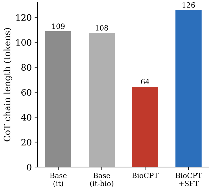
CPT shortens the reasoning chain
