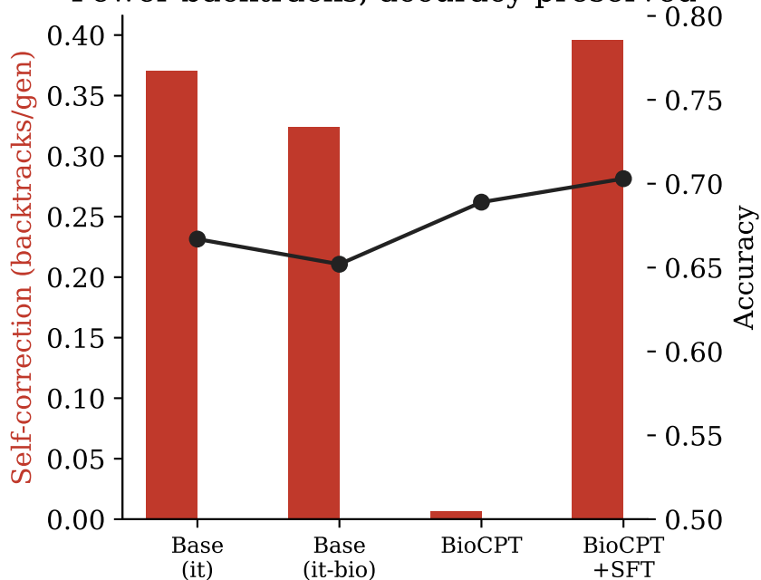
Fewer backtracks, accuracy preserved
