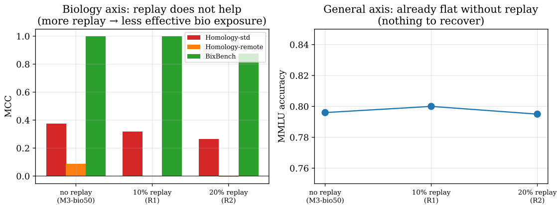
Figure 8: Replay control. Left: the biology axis does not benefit from end-of-training text replay and mildly declines as replay fraction rises. Right: the general axis is already flat without replay, so there is nothing for replay to recover.
