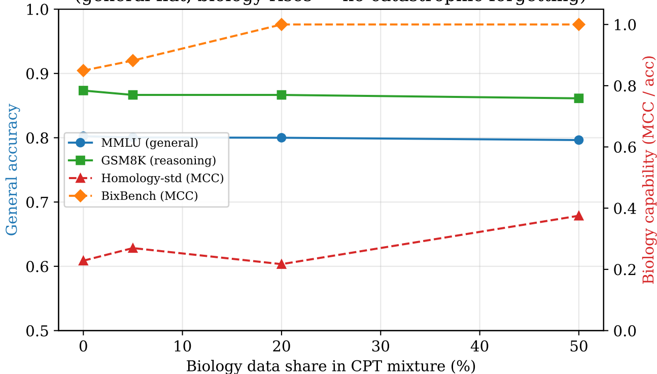
Capability shaping by biology mixture ratio (general flat, biology rises — no catastrophic forgetting)
