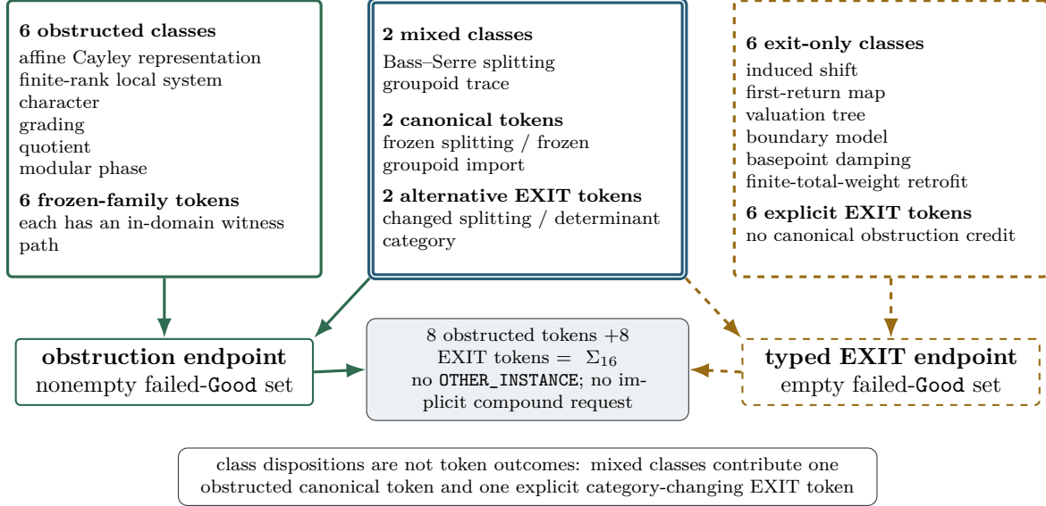
Figure 2: The finite classifier separates class dispositions from token outcomes. Six classes are obstructed and six are exit-only. Each of the two mixed classes contributes one obstructed canonical token and one explicit category-changing exit token. Thus the token census is eight plus eight. Solid paths terminate with a nonempty failed-Good set; dashed EXIT paths terminate with an empty set and never count as evidence for \neg \text{Good} .
