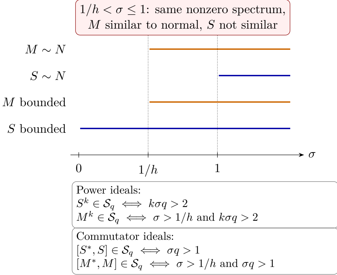
Figure 2: Exact existence, similarity, power-ideal, and commutator-ideal conditions. The horizontal bands encode only the fixed ordering 0 < 1/h \leq 1 ; the ideal thresholds are stated algebraically because their relative positions depend on h, k, q . Every displayed wall is strict.
