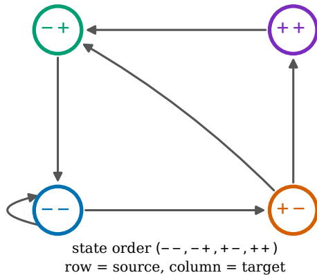
(b) six allowed transitions
