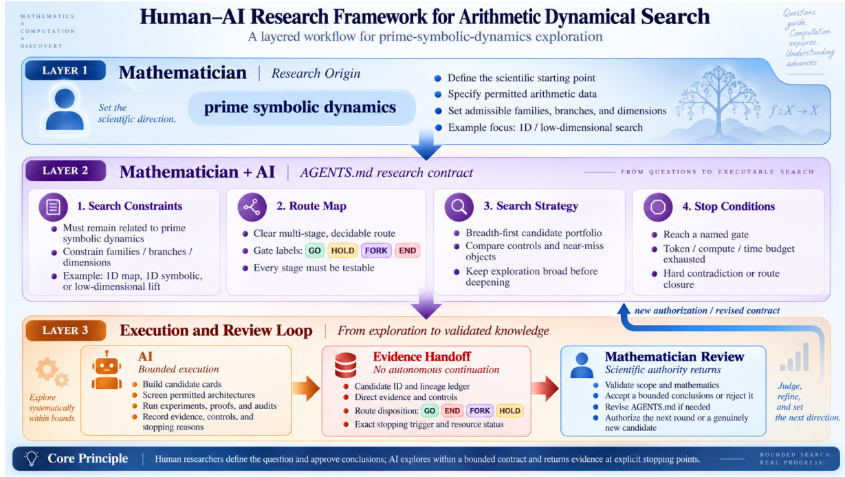
Figure 1: Three-layer human–AI research framework for arithmetic-dynamical search. Layer 1: the mathematician fixes the prime-symbolic origin and permissible search envelope. Layer 2: a jointly drafted, human-approved AGENTS.md fixes constraints, a testable route, a breadth-first portfolio with controls and near misses, and stopping conditions. Layer 3: bounded AI execution, evidence handoff, and mathematician review; continuation needs a new authorization or revised contract. GO, HOLD, FORK, and END are unordered workflow dispositions, not Route-A/Route-B passes. This is a prospective Round-2 framework, not a claim that Phase-I sessions used one uniform agent protocol.
