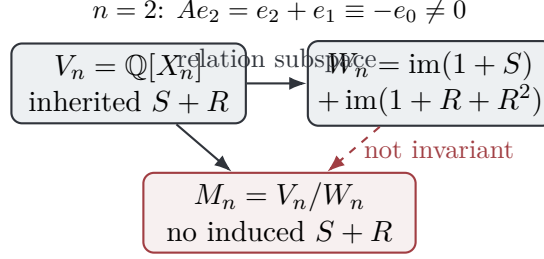
Figure 3: The relation quotient kills the intended boundaries, but the original S + R adjacency sends a relation vector outside the relation subspace on the n = 2 block. Replacing it by a scalar homology operator changes the marker and forfeits same-object determinant ownership.
