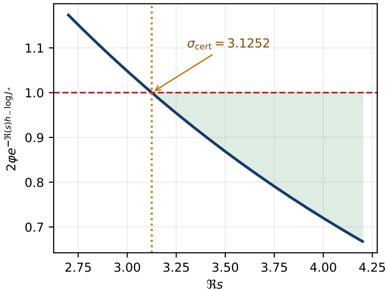
Certified all-orbit contraction
