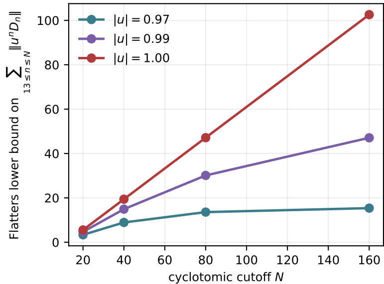
One-orbit Abel boundary
