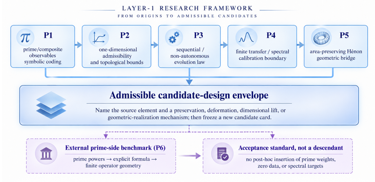
Figure 3: Layer-1 research origin and candidate-design boundary. P1–P5 are an internal conceptual genealogy from the prior-work guide; P6 is a distinct prime-side benchmark. The arrows express research provenance and admission constraints, not theorem implications, Route transfer, or evidence that a proposed descendant already has a prime-dynamical realization.
