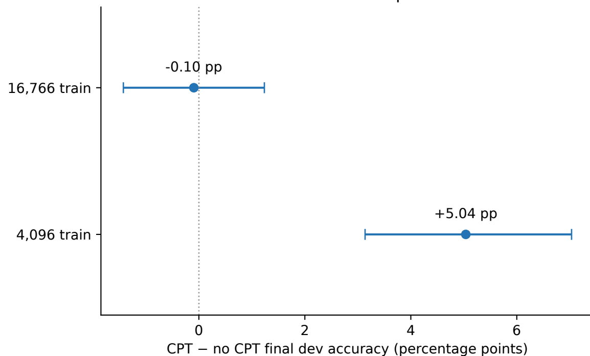
D. Paired difference with descriptive 95% intervals
