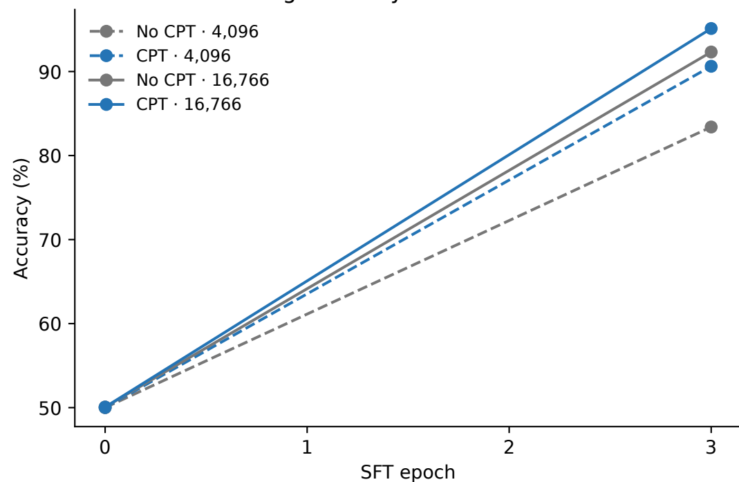
C. Training accuracy before and after SFT
