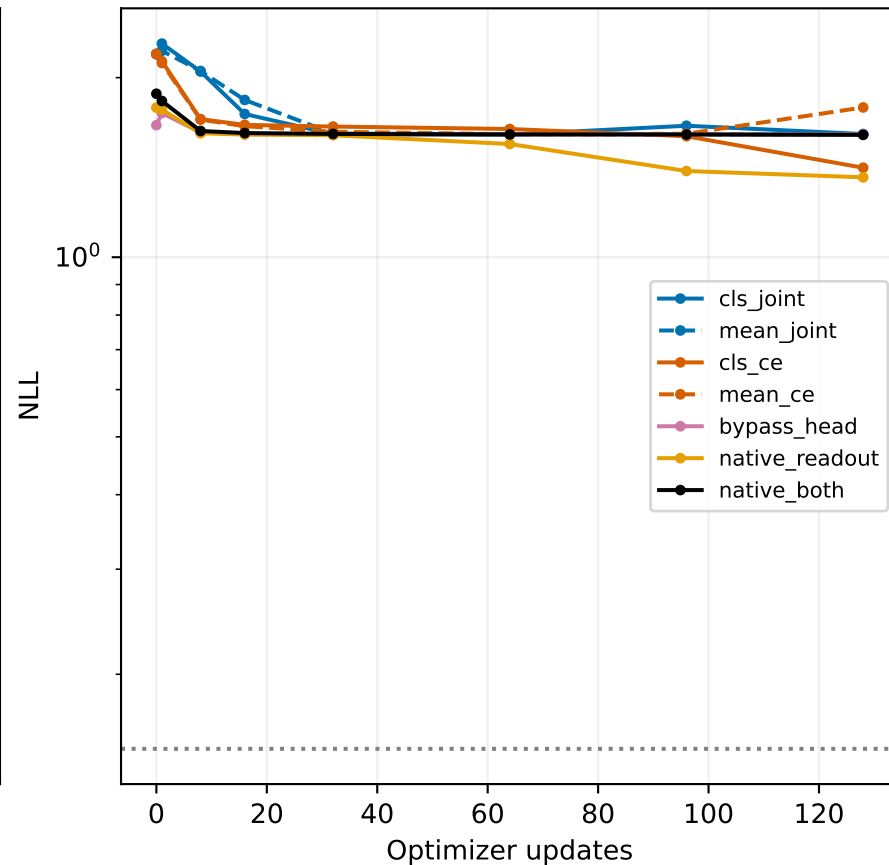
Supervised five-bin classification
