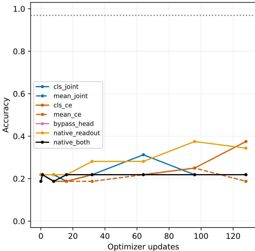
Supervised five-bin classification
