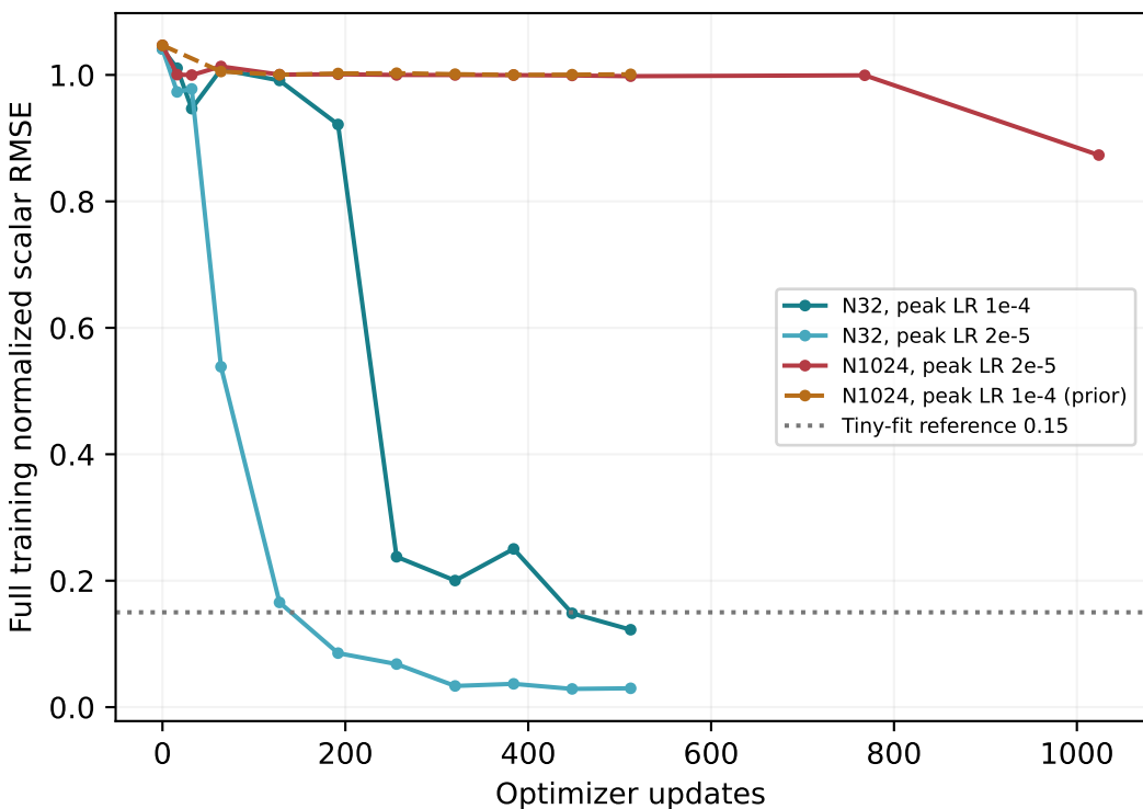
Training-only GFP scale / learning-rate probe; one seed
